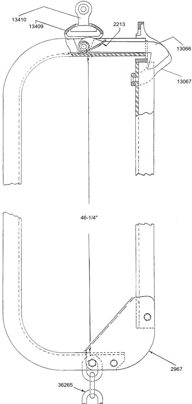
438680 Stanchion Complete, 7-8"
